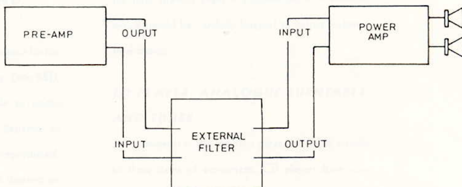
PERMANENT CONNECTION
