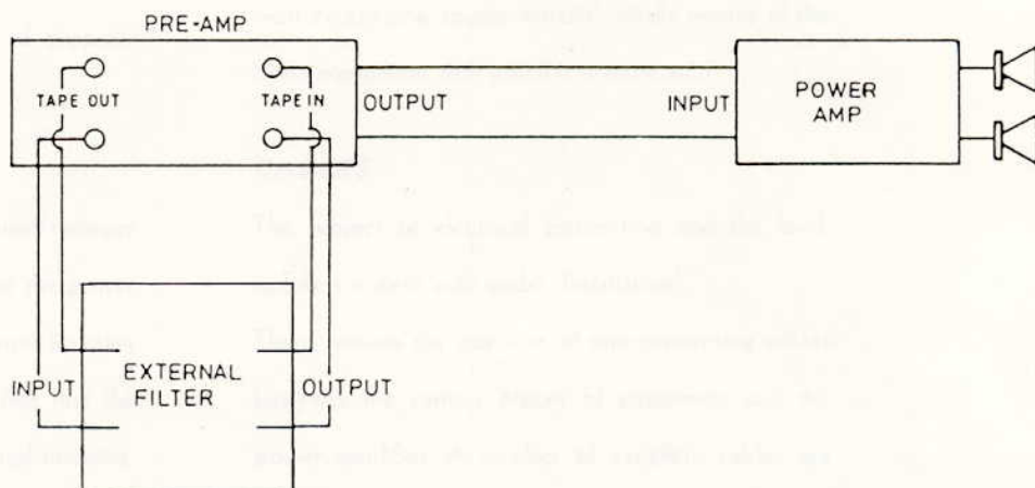
SWITCHED CONNECTION
